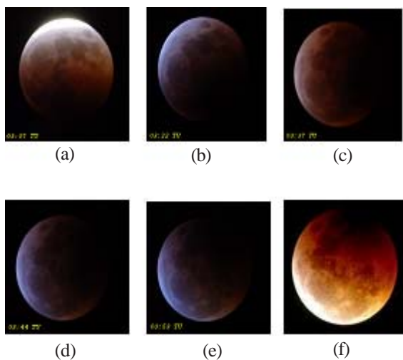
Figure 3: Selected photos of the totally eclipsed Moon (courtesy of WCS and JCD)
