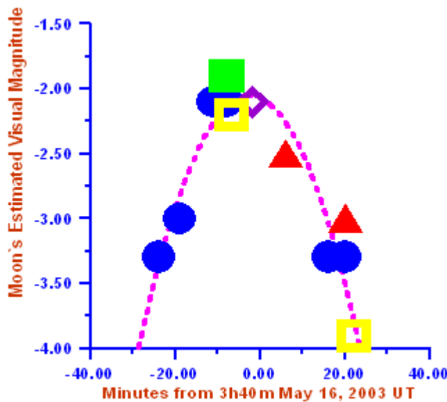
Figure 5: Visual magnitude estimates of the Moon
