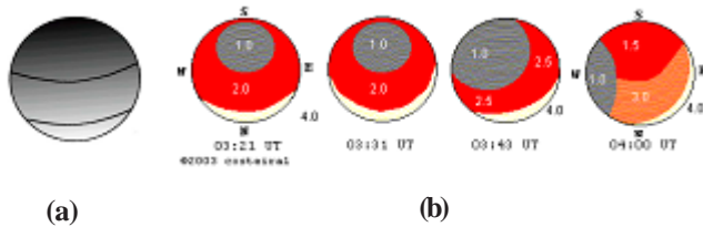
Figure 2: (a) Brightness distributions observed by HCV and (b) by AA (courtesy of Costeira 15 ) (south is up)
