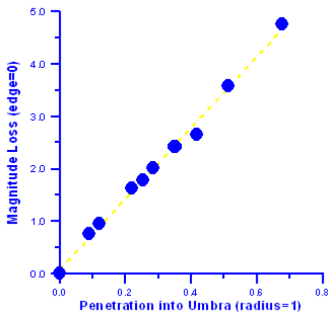
Figure 6: Magnitude loss with penetration into the umbra
