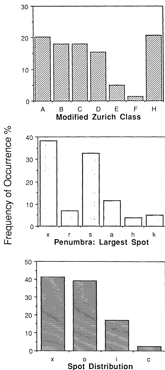
Fig. 2. Frequency of occurrence of the 17 categories within the McIntosh classification. Data from Kildahl (1980).
